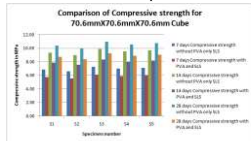
Comparison of compressive strength of concrete for 70.6X70.6X70.6 size specimen
