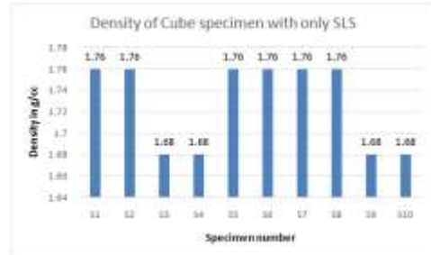
Density of 50mmX50mmX50mm cube only with SLS
