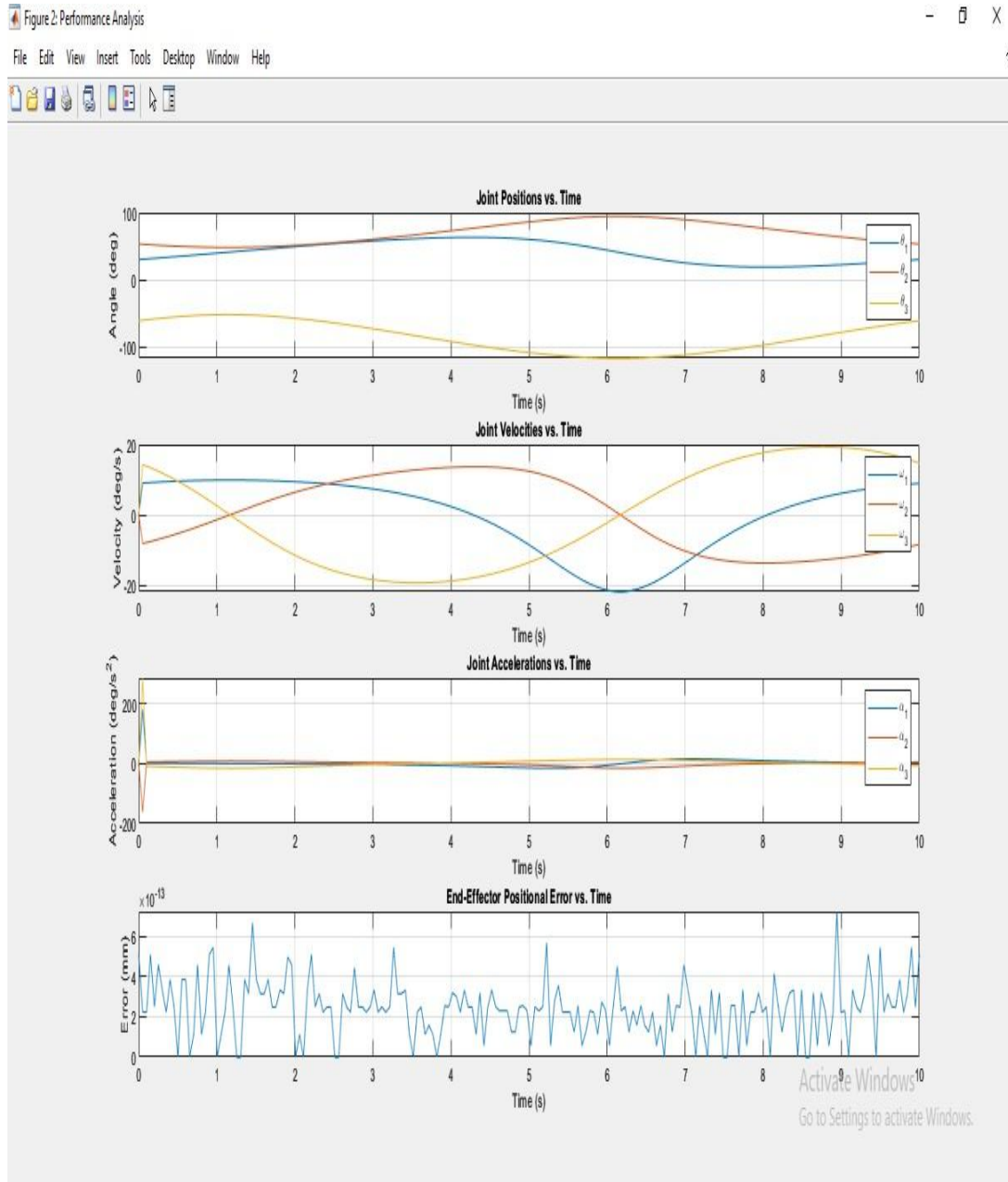
Graph 4:3dof robotic arm performance kinematic analysis results
