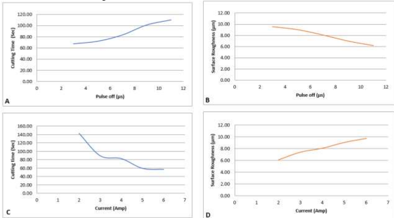
Fig.13 (A) The effect of Pulse off on Cutting Time (B) The effect of Pulse off on Surface Roughness (C) The effect of Current on Cutting Time (D) The effect of Current on Surface Roughness
