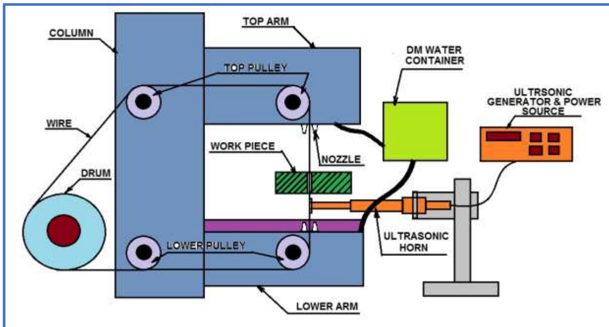
Fig. 3 Ultrasonic-Assisted Electric Discharge Machining Schematic Diagram
