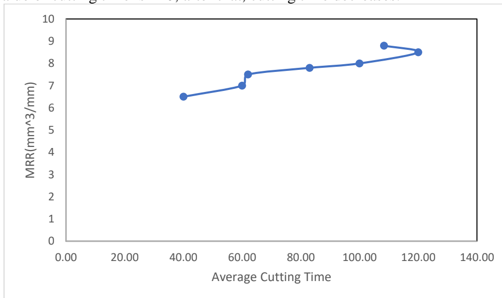
Fig.12 The effect of amplitude of average cutting time on MRR
