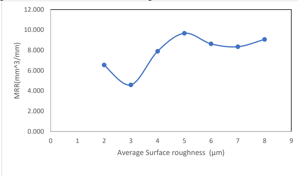
Fig.11 The effect of amplitude of average surface roughness on MRR
