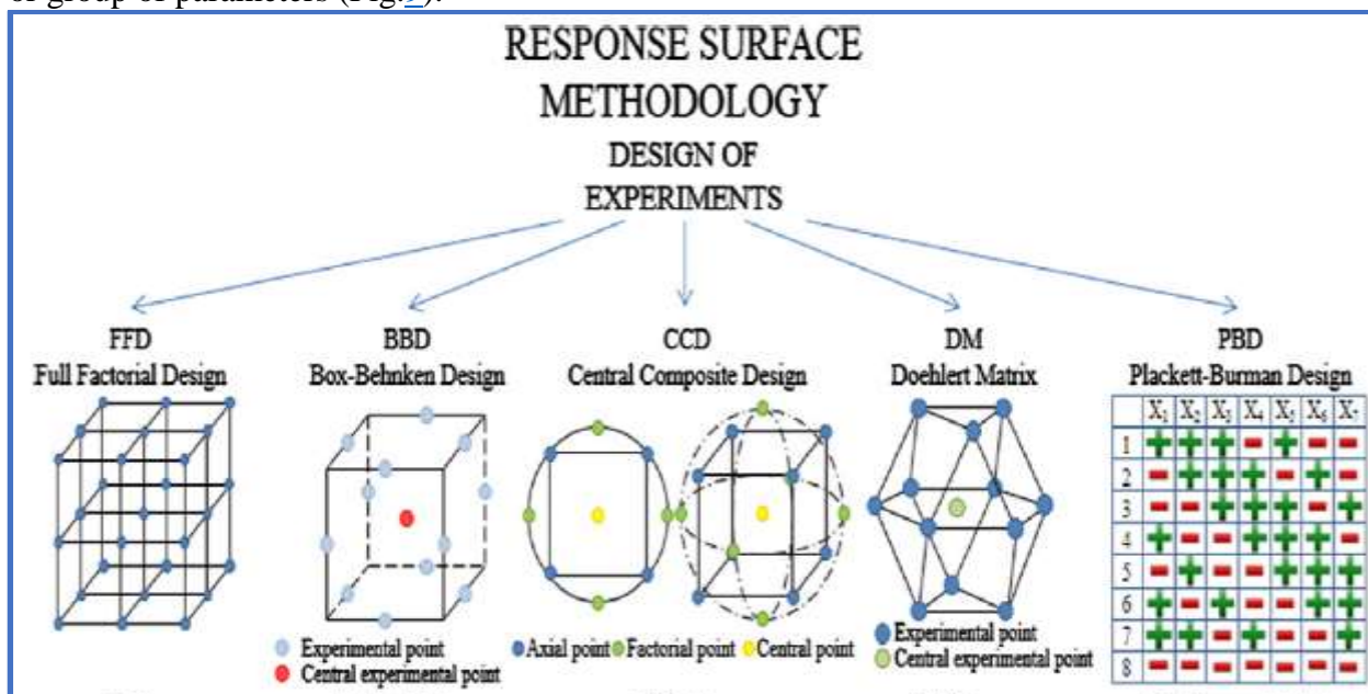
Fig. 9 Response Surface Methodology
