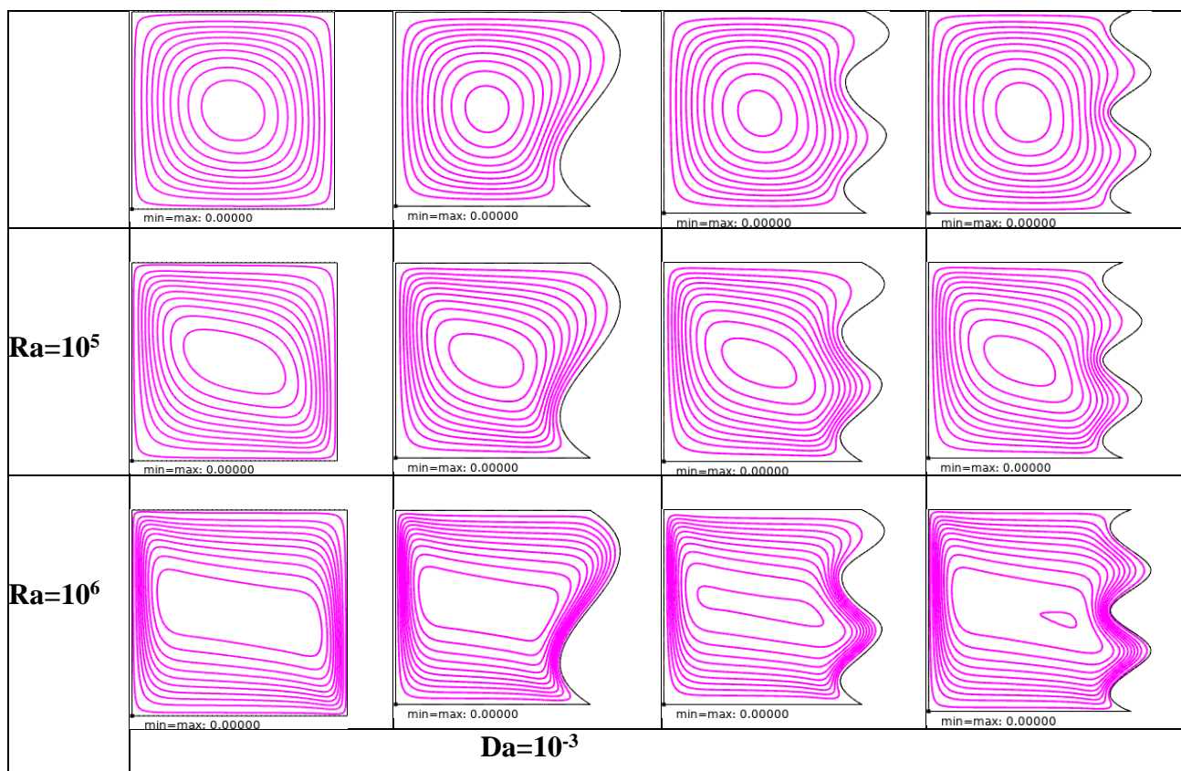
Fig5. Streamlines at da=10^{-3} with different undulations from ( d=0 to d=3 ) and Rayleigh number 10^3 \leq Ra \leq 10^6 sinusoidal wall case.
