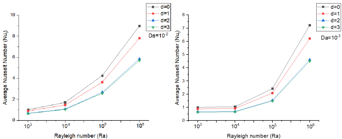
Fig 15. Average Nusselt number variations w.r.t different undulations from ( d=0 to d=3 ) for sinusoidal side wall and Rayleigh number Ra=10^3 to 10^6 at (a) DA=10^{-2} (b) DA=10^{-3} (c) DA=10^{-4} . Fig. 16 shows the variation of Nu_t with respect to Ra for different undulation ( d=0, 1, 2, 3 ) and different \phi , for zig zag side wall case. In this for each \phi , the Nu_t value for zig zag side wall when d=0 increases with Ra , while for d=1, 2, 3 undulations, the Nu_t value is lower than that of d=0 case. This is because the undulation causes increase in flow resistance in flow path, this increased resistance may result in reduced fluid flow and heat transfer rate, which leads to lower value of Nu_t .
