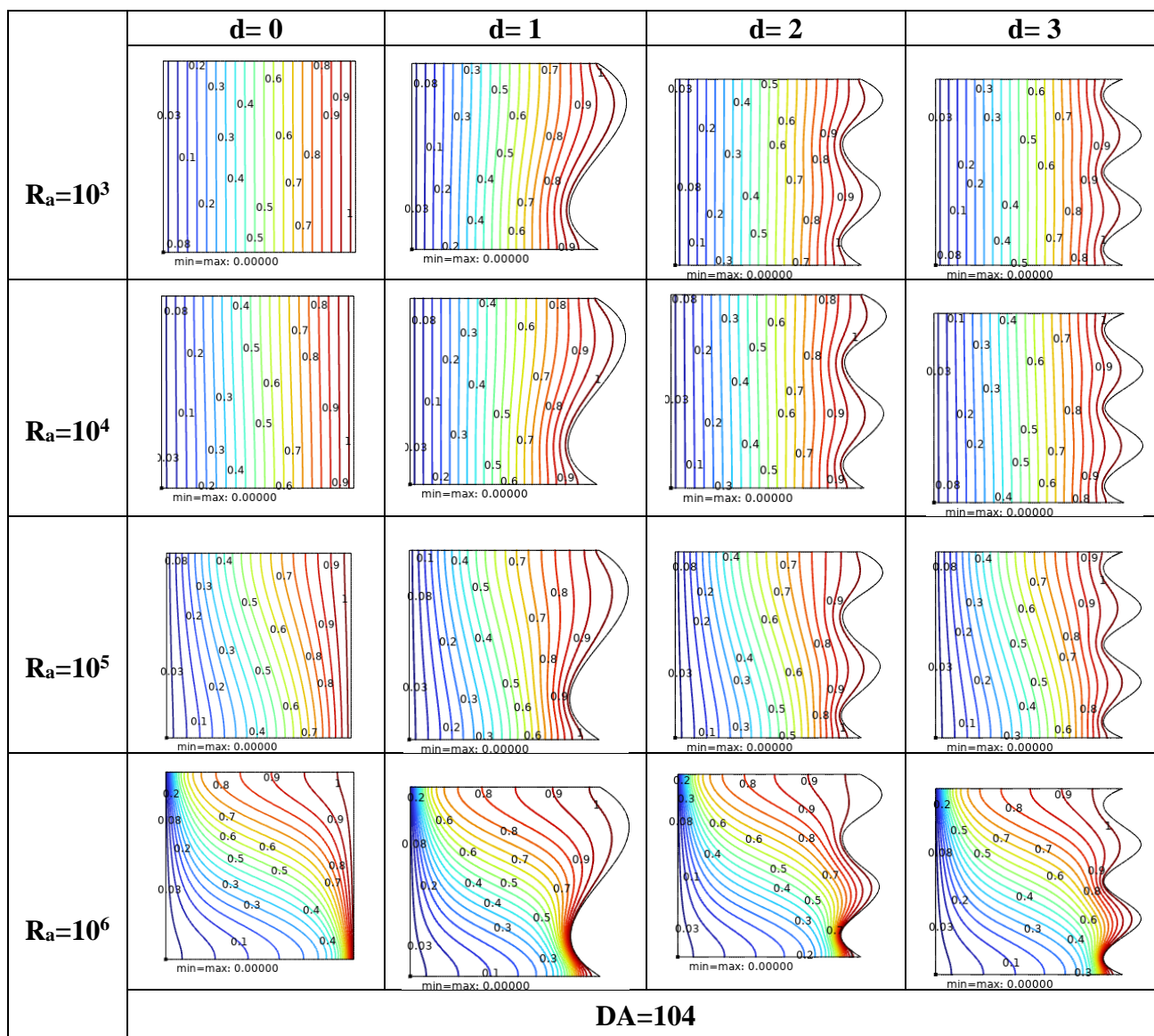
Fig 4. Isotherms at da=10^{-4} with different undulations from ( d=0 to d=3 ) and Rayleigh number 10^3 \leq Ra \leq 10^6 sinusoidal wall case.
