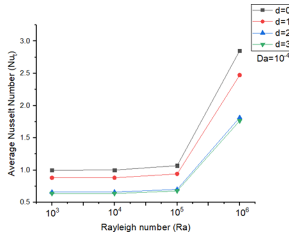
Fig 16. Average Nusselt number variations w.r.t different undulations from (d=0 to d=3) for zig zag side wall and Rayleigh number 10^3 \leq Ra \leq 10^6 at (a) DA=102 (b) \phi 3\% (c) DA=104
