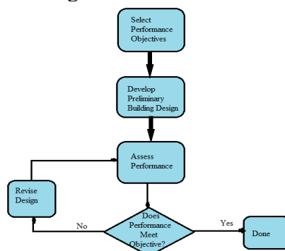
Figure 2 – Flow chart of performance based design
