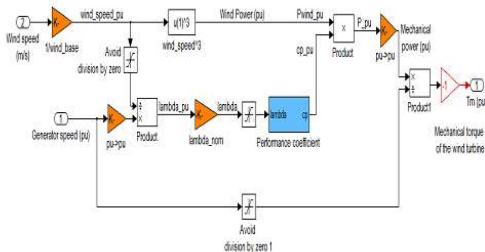
Figure 7: Implementation of Wind Turbine System
