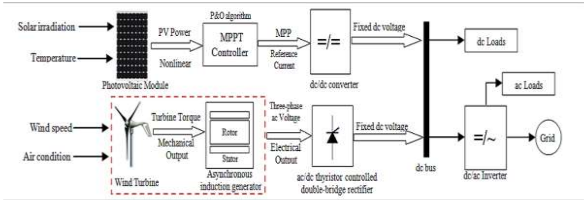
Fig 1: Basic architecture of Hybrid System
