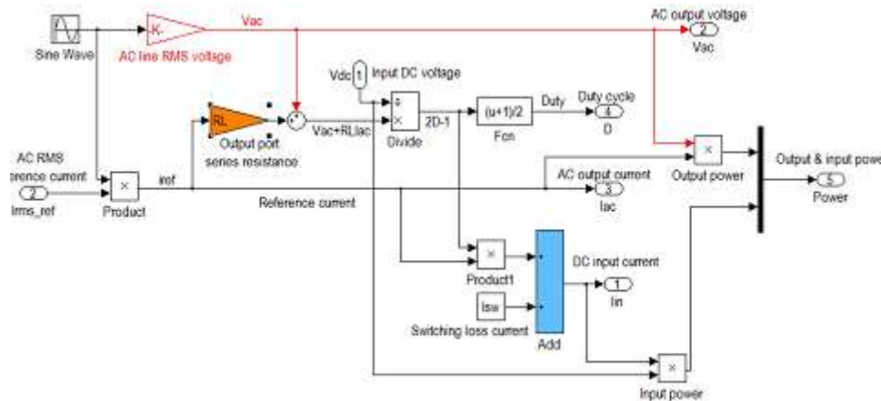
Figure 8: Control Diagram for Power management strategy in Hybrid System
