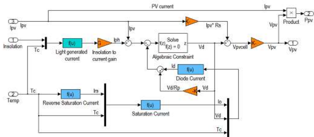
Figure 3: Control Diagram for PV System
