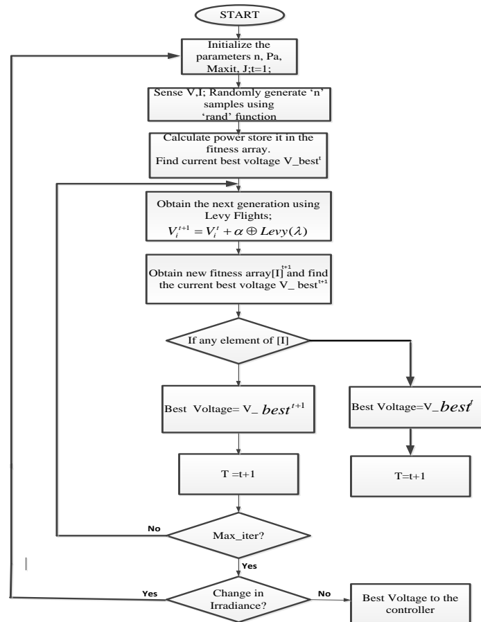
Figure 4: Cuckoo Search Algorithm
