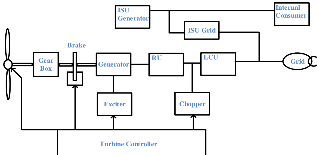
Figure 5: Basic Wind Turbine System
