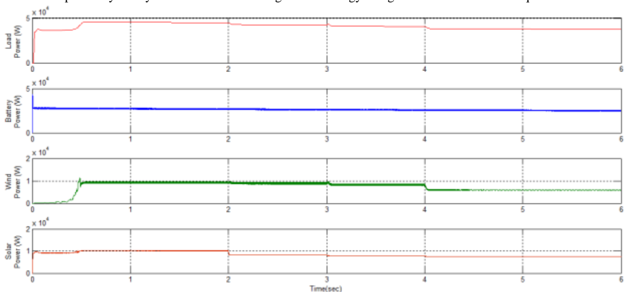
Figure 9: Simulation Result for (a) Load Demand, (b) Solar Power, (c) Grid Power and (d) Battery Power
