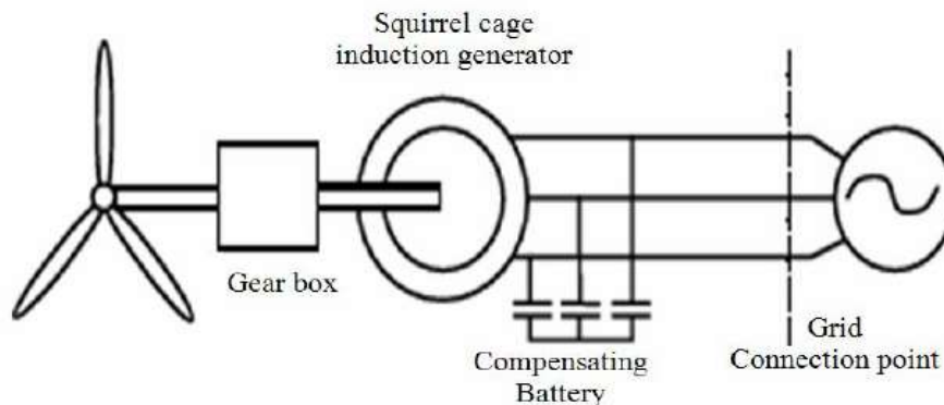
Figure 6: SCIG based WES
