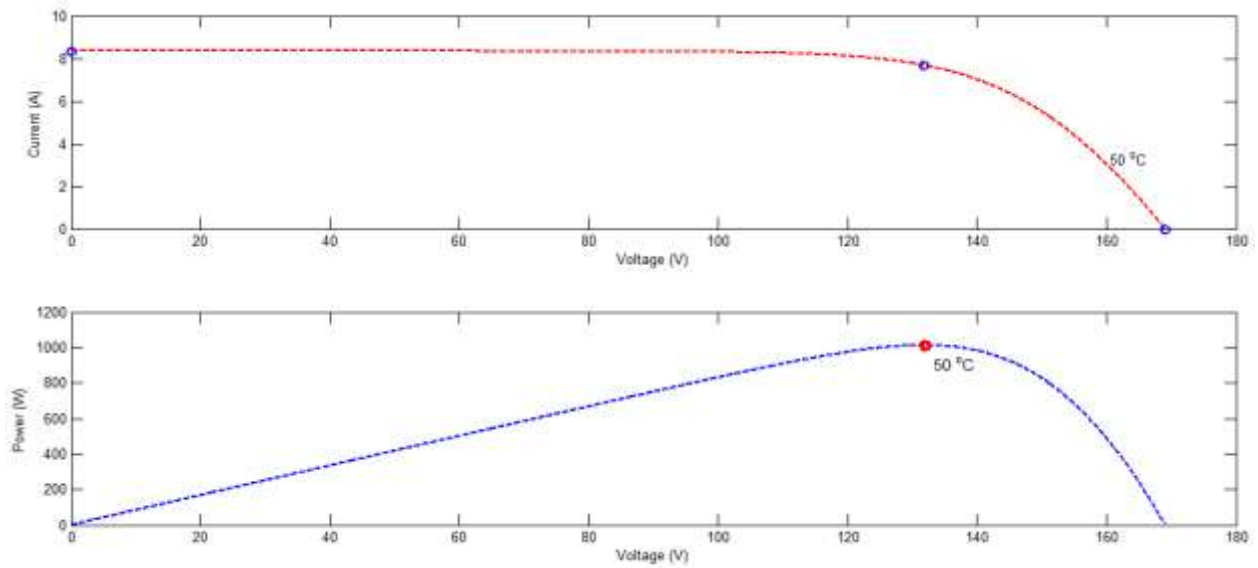
Figure 3: V-I Characteristics of PV system
