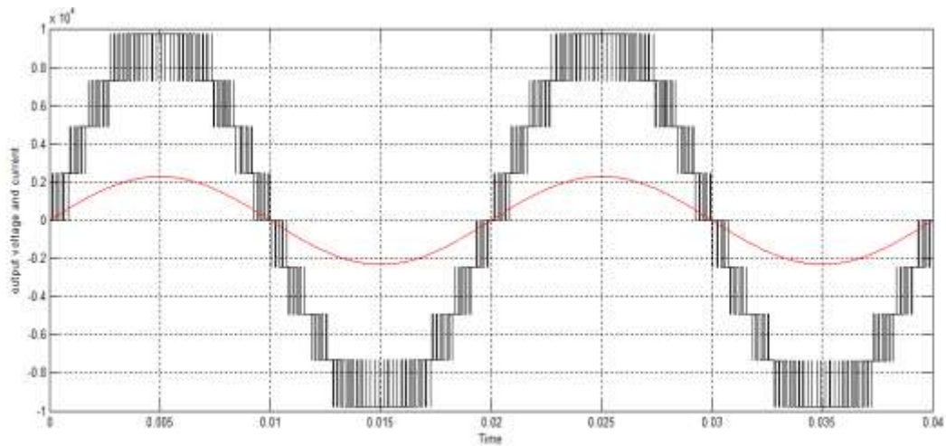
Fig 7: Output Current and voltage
