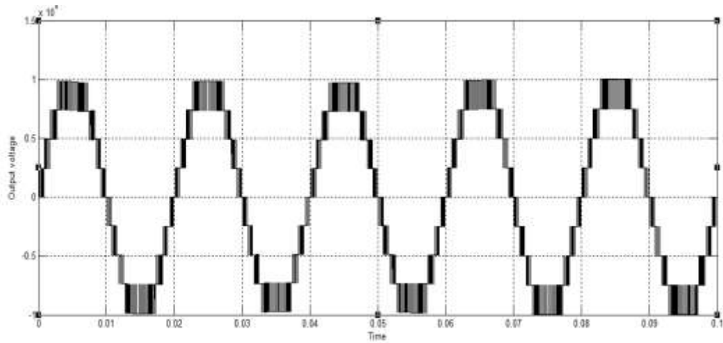
Fig 8: Nine Level Output Voltage
