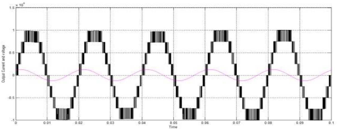
Fig 9: Output Current
