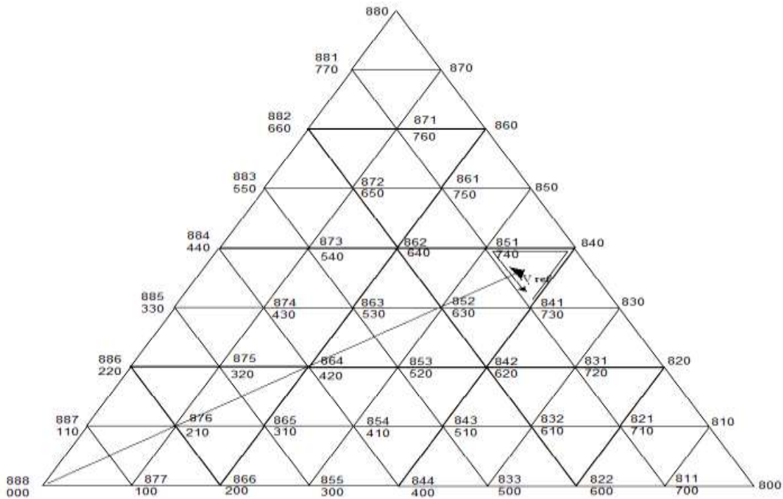
Fig 3: vector diagram for 9Level converter
