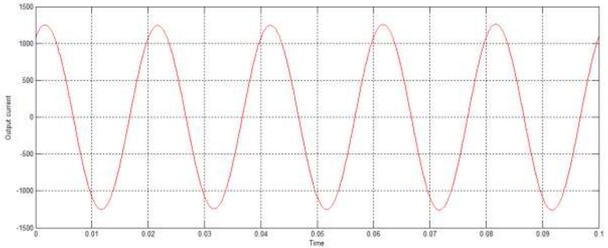
Fig 9: Output Current
