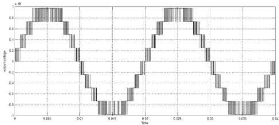
Fig 4: Simulation Diagram for the ANPC system
