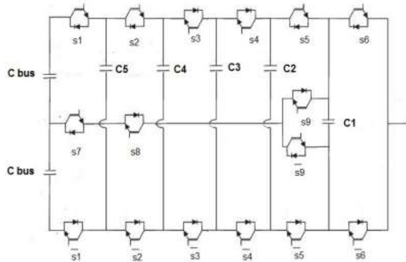
Fig 1: Proposed Nine-Level ANPC configuration
