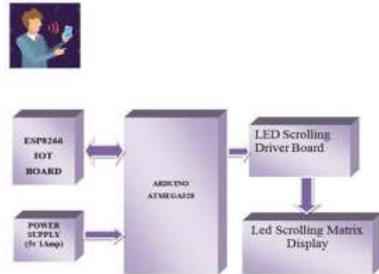
Fig 2. Block Diagram
