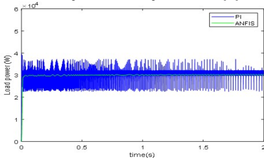
Fig 12: Load Power Vs Time Waveform
