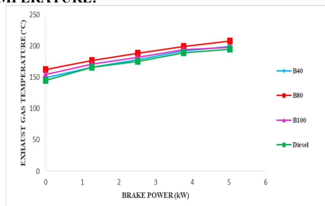
Fig.3: Exhaust gas temperature with BP
