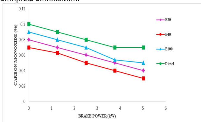
Fig.4: Carbon monoxide variation with load
