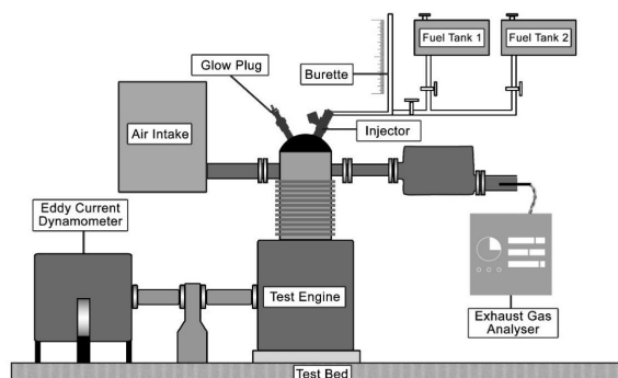
Fig.1: Experimental Setup
