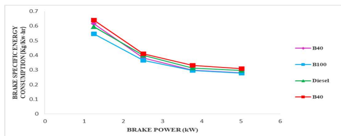
Fig.2: Fuel consumption and Brake power
