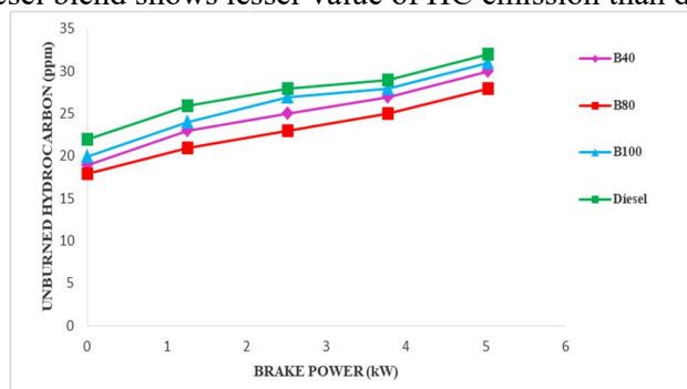
Fig. 6: UHC with load
