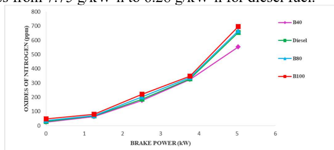
Fig. 5: NO x Emission with load
