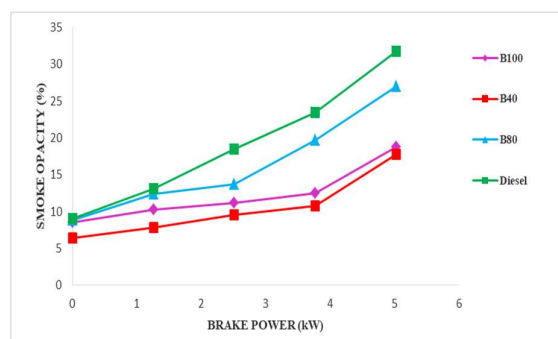
Fig.7: Variation of smoke with BP
