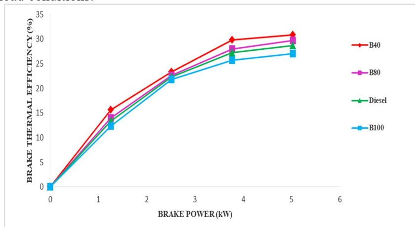
Figure 1 BP vs BTE
