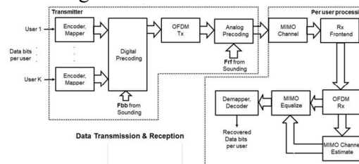
Fig. 1. Model for Data Transmission and Reception in MIMO-OFDM Systems
