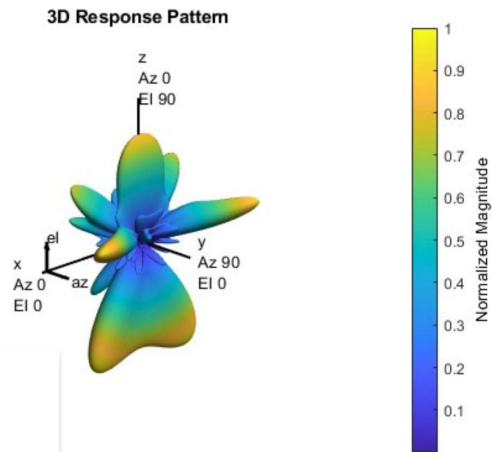
Fig. 4. Radiation Pattern for 256-QAM Modulation Scheme for Scattering Channel at Carrier Frequency of 6 GHz
