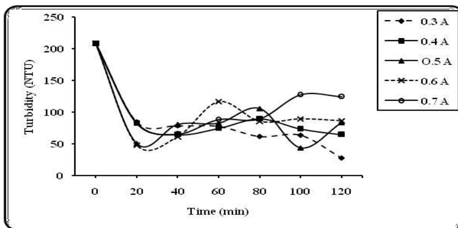
Figure-07: Current Intensity from 0.3A to 0.7A on Turbidity
