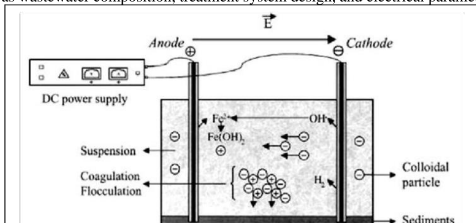
Figure-03: Principle of Electro-coagulation
