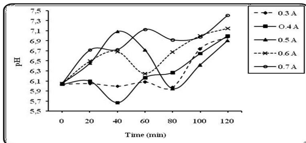
Figure-05: Current Intensity from 0.3A to 0.7A on pH Solution.
