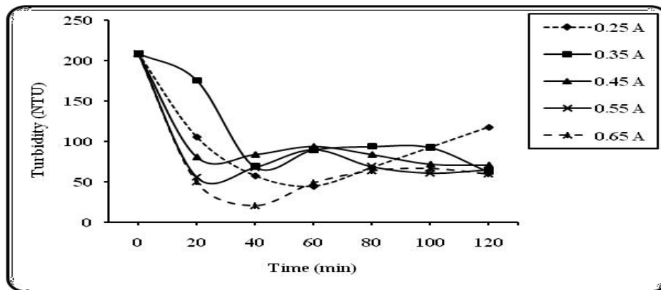
Figure-06: Current Intensity from 0.25A to 0.65A on Turbidity.
