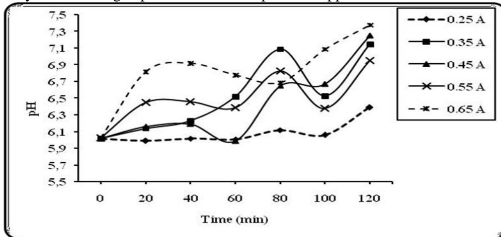
Figure-04: Current Intensity from 0.25A to 0.65A on pH Solution.
