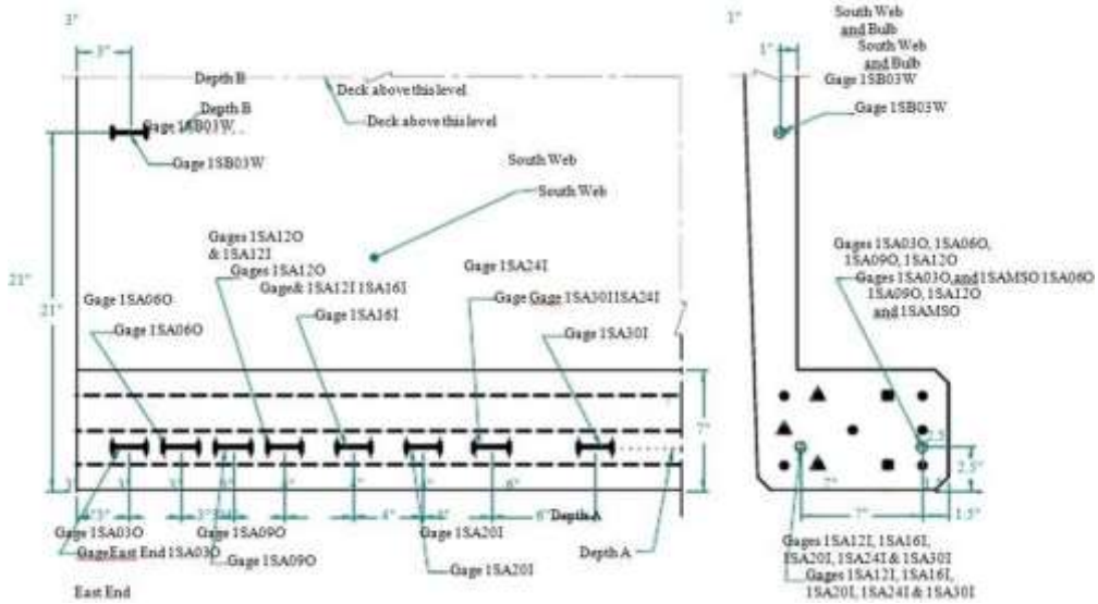
Fig 3: Instrumentation plan for vibrating wire gauges
