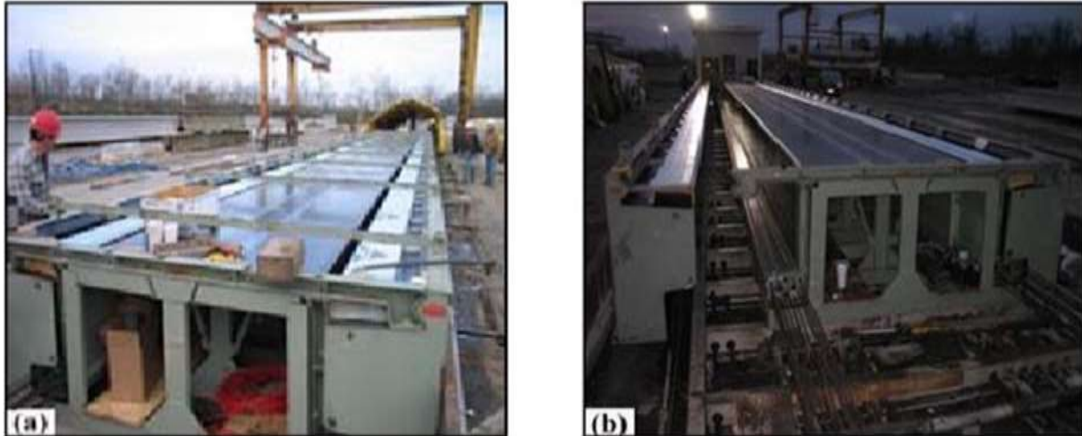
Fig 5: girder framework
