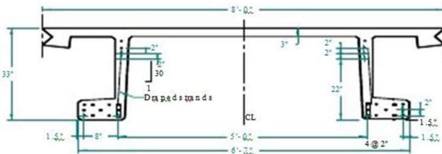
Fig 2:Girder section details
