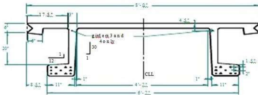
Fig 1: Section details for girders 1,2,3 and 4
