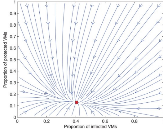
Fig 4: The parse portrait of the system Under the given example
