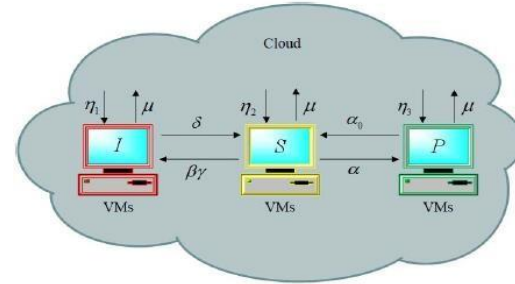
The Transfer Diagram Of The Proposed Dynamical Propagation Model Of Malware
