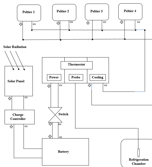
Fig. 10 Circuit Diagram
