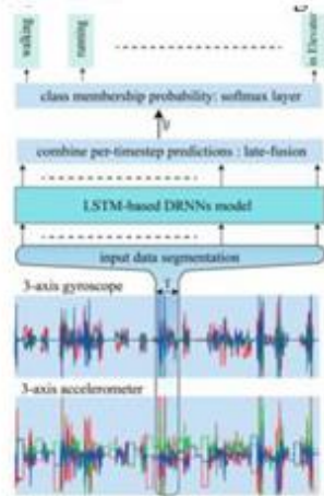
Figure 3. The LSTM based model proposed in [34] that utilizes accelerometer and gyroscope data.
