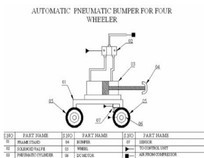
Drawing For Automatic Pneumatic Bumper for Four Wheeler:
