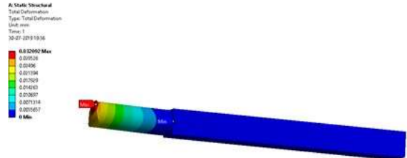
Figure9 TOTAL DEFORMATION AT FORCE 150N
