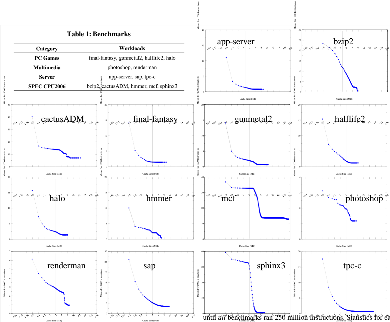
Figure 4: Cache Sensitivity of Workloads Used in this Study.
