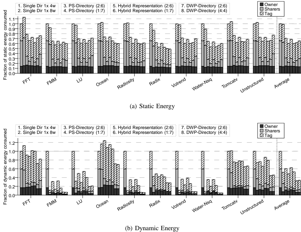
Fig. 8: Normalized energy consumed with respect to a single-cache directory with 4 ways and 32 cores
