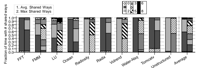
Fig. 2: Fraction of time with # shared entries in a set.
