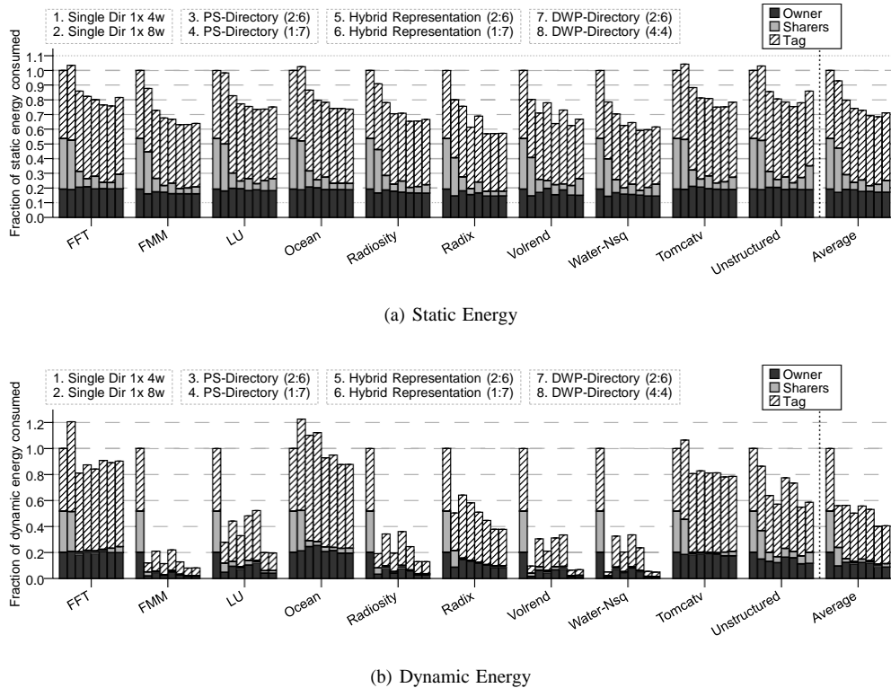
Fig. 7: Normalized energy consumed with respect to a single-cache directory with 4 ways and 16 cores
