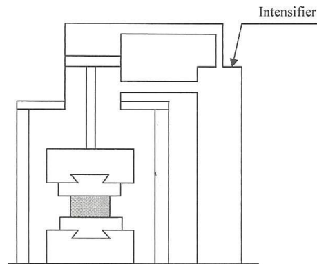
Figure 5: Hydraulic press
