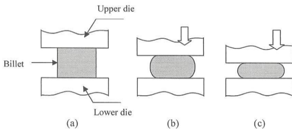
Figure 1: Open-die forging
