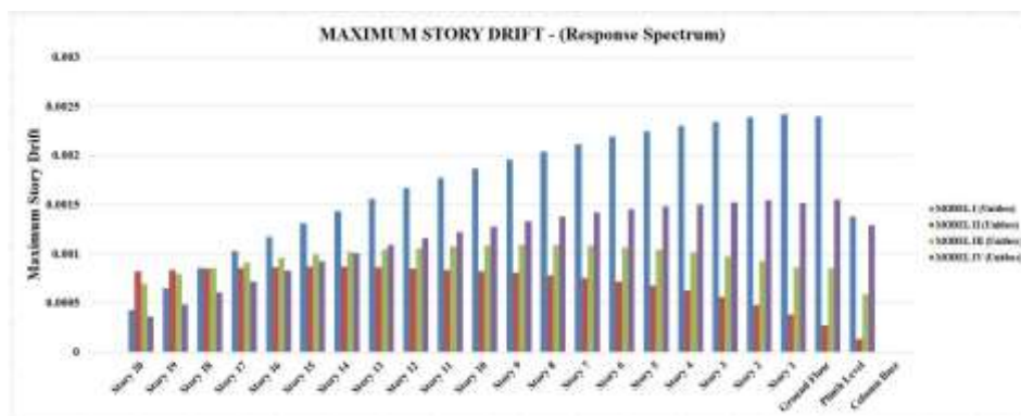
Fig 17. Comparison graph of Maximum Story Drift
