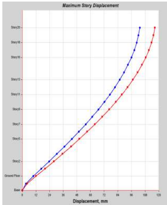
Fig 15. Maximum Story Displacement of Model I
