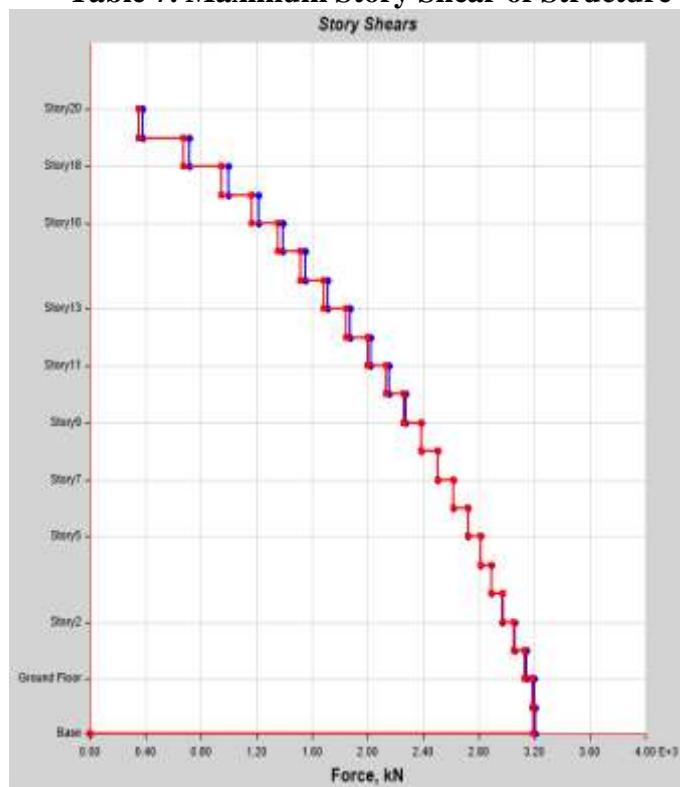
Fig 19. Maximum Story Shear of Model I
