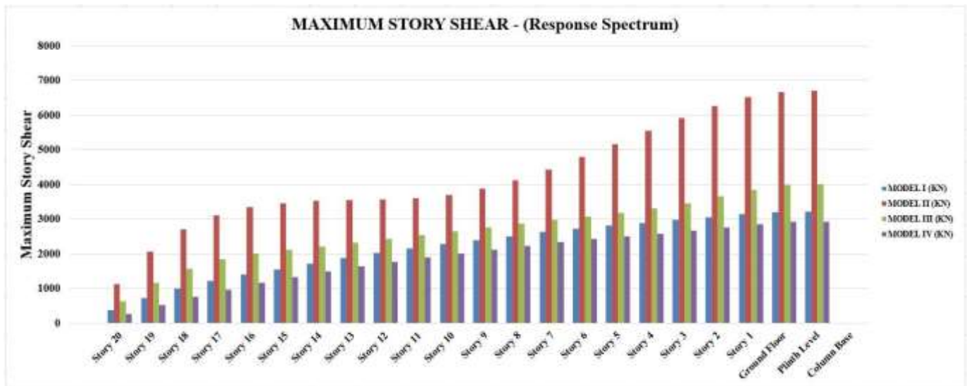
Fig 20. Comparison graph of Maximum Story Shear
