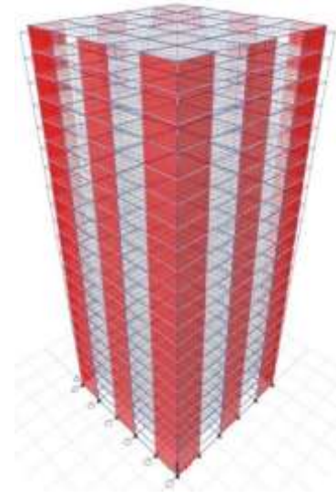
Fig 12. Deformation of Model II
