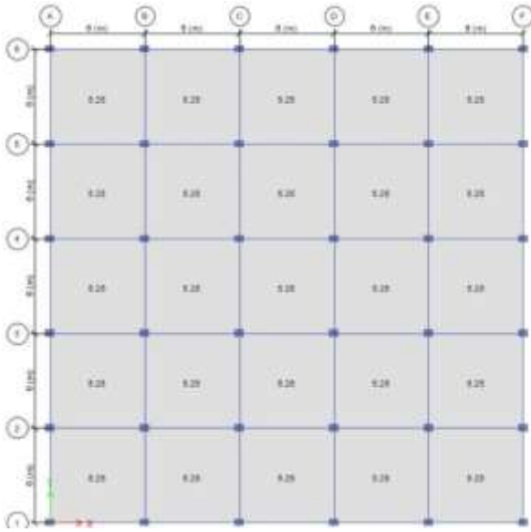
Fig 5. Dead Load on Slab
