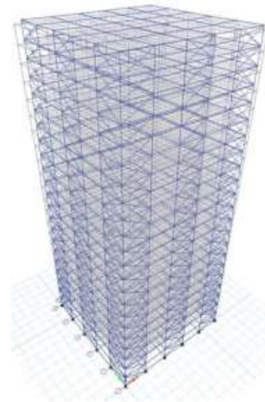
Fig 14. Deformation of Model III
