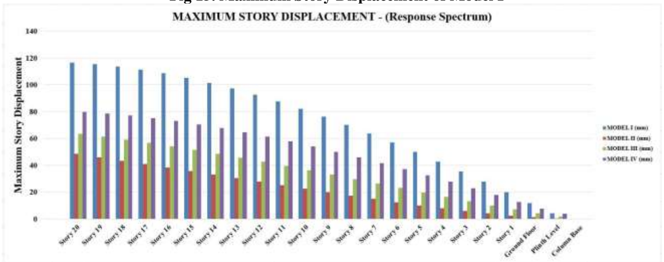
Fig 16. Comparison graph of Maximum Story Displacement 5.1.2 MAXIMUM STORY DRIFT- (Response Spectrum) ZONE V
