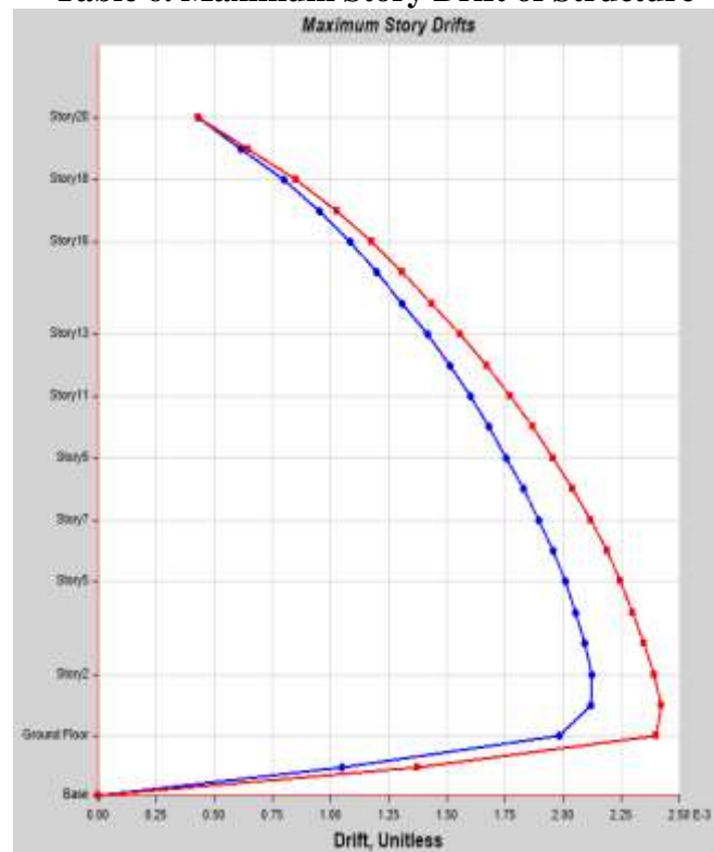
Fig 18. Maximum Story Drift of Model I
