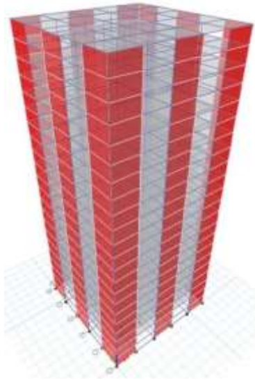
Fig 11. 3D View of Model II
