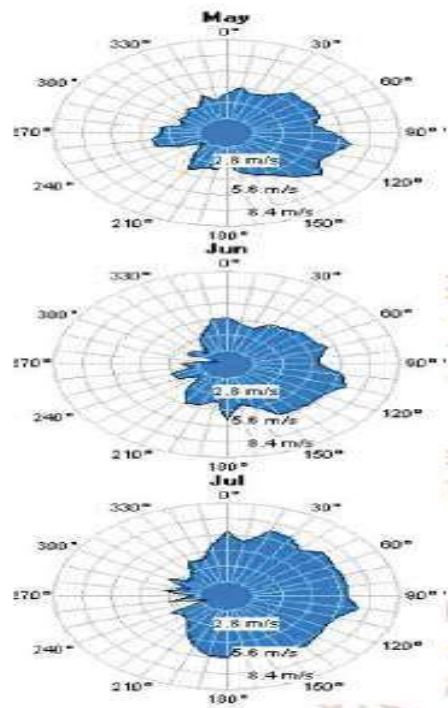
Fig.6. Wind Analysis
