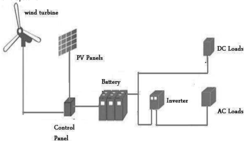
Fig.4. Hybrid Systems
