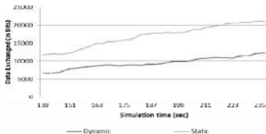
Fig. 6 Data Exchanged in number of bits
