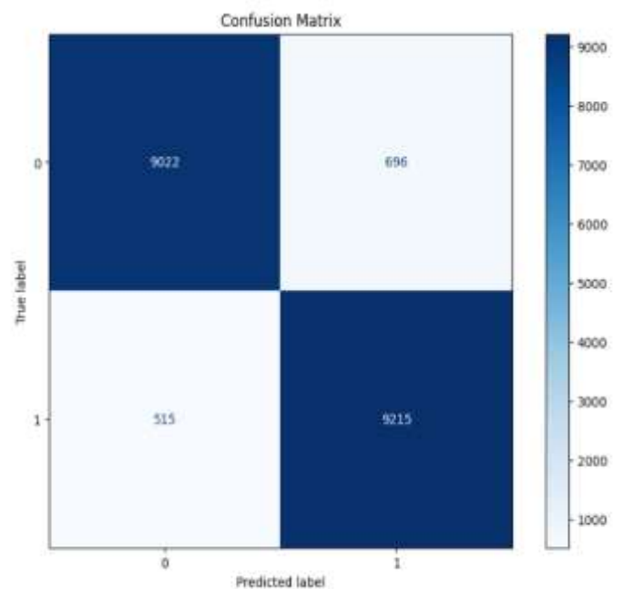
Fig 3: Confusion Matrix of Random Forest
