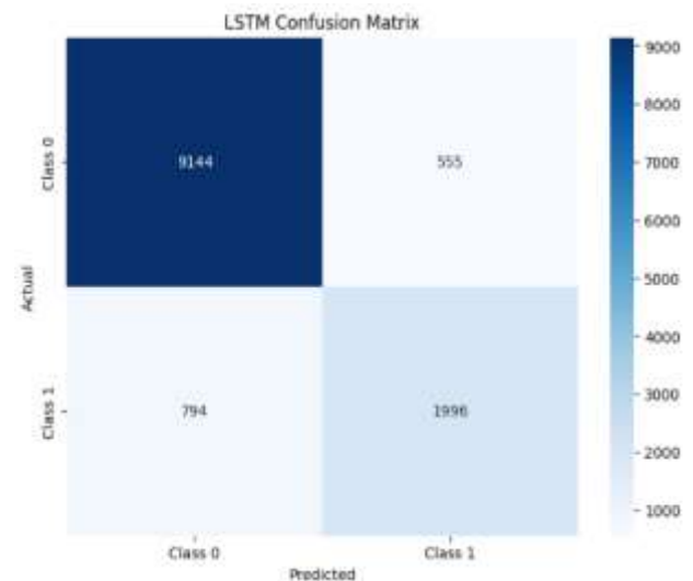
Fig 6: Confusion Matrix of Long Short-Term Memory (LSTM)
