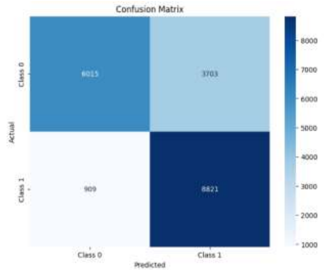
Fig 4:Confusion Matrix of Naive Bayes
