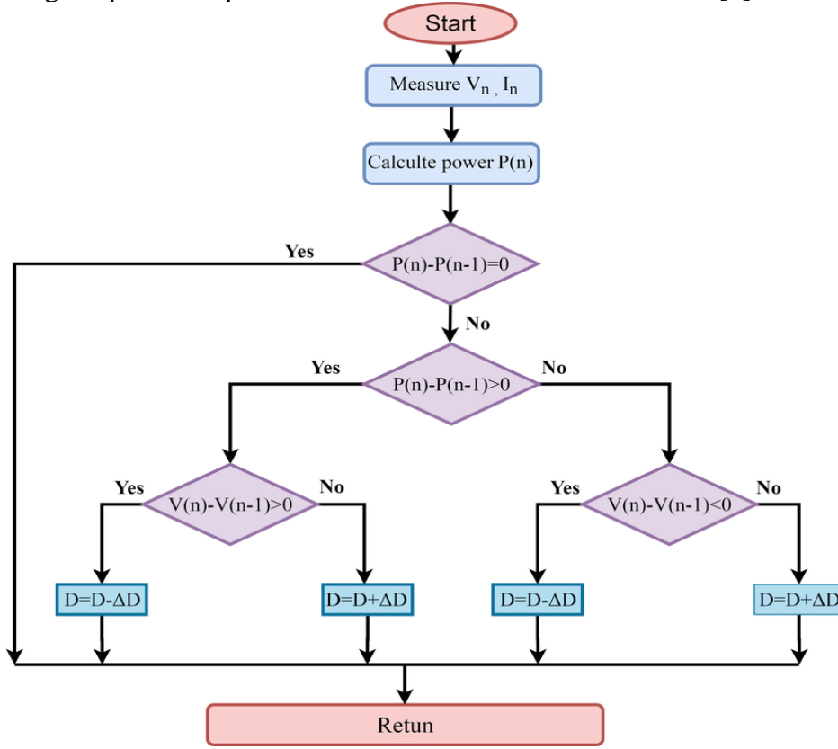
Figure 5-P&O Algorithm
