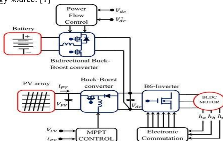
Figure 1- Solar PV System with A Battery and BLDC Motor
