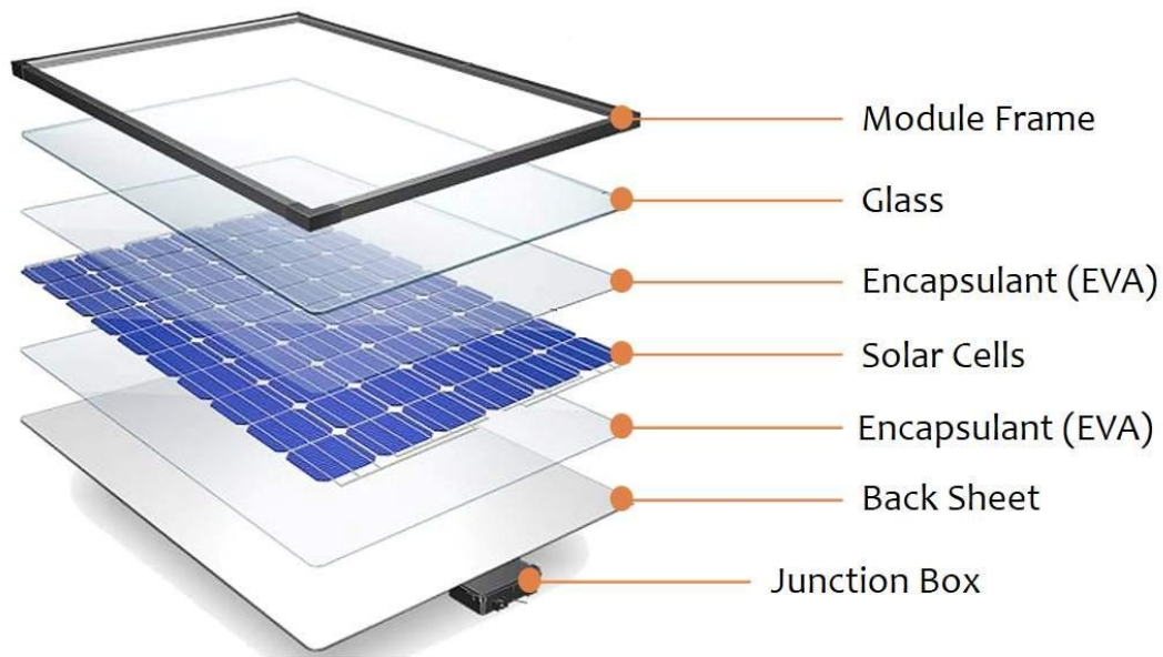
Figure 3-solar PV panel
