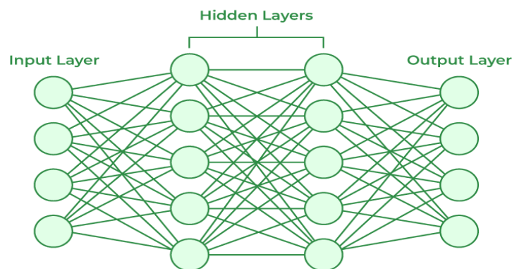
Figure 7-artificial neural network
