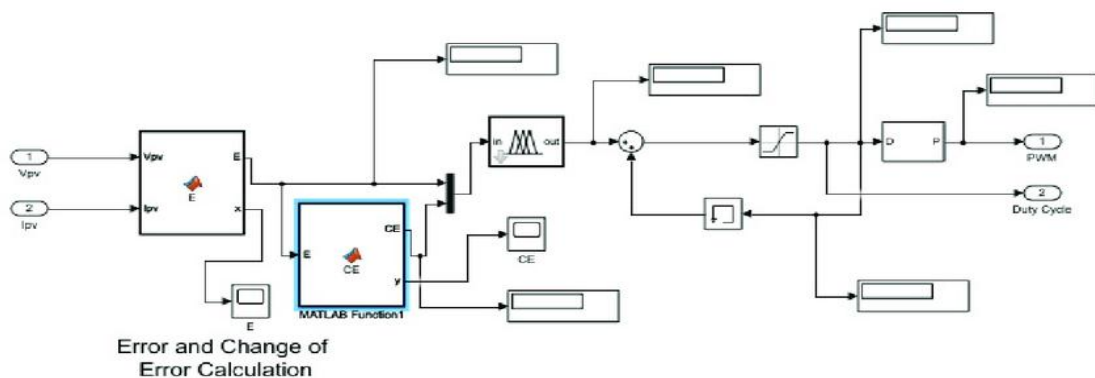
Figure 10-Hybrid ANN fuzzy Logic System For MPPT
