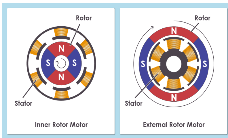
Figure 4- BLDC Motor
