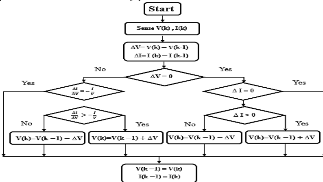
Figure 6-INC algorithm
