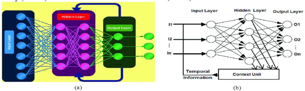
Figure 9-Recurrent Neural Network architecture for MPPT
