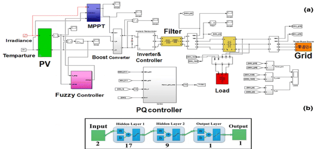
Figure 8-Feedforward Neural Network architecture for MPPT
