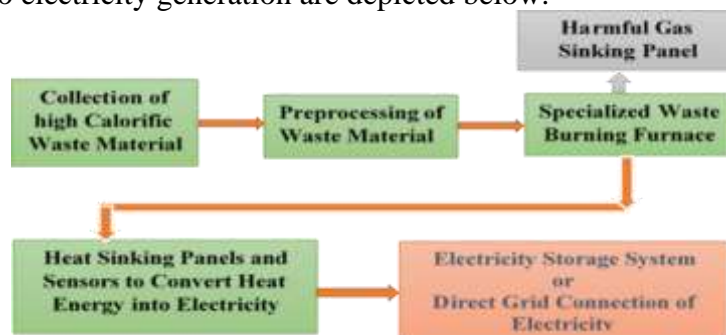
Figure 2: Methodology used to generate electricity from waste material
