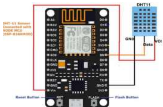
Figure 4: Block diagram and connections
