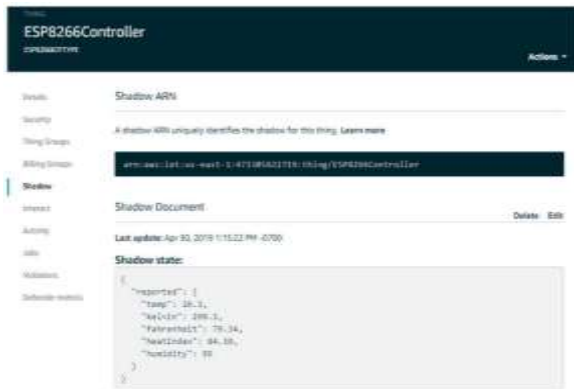
Figure 8: AWS IoT Core Shadow
