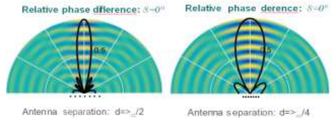
Fig. 3. Comparison of antenna separation scenarios.
