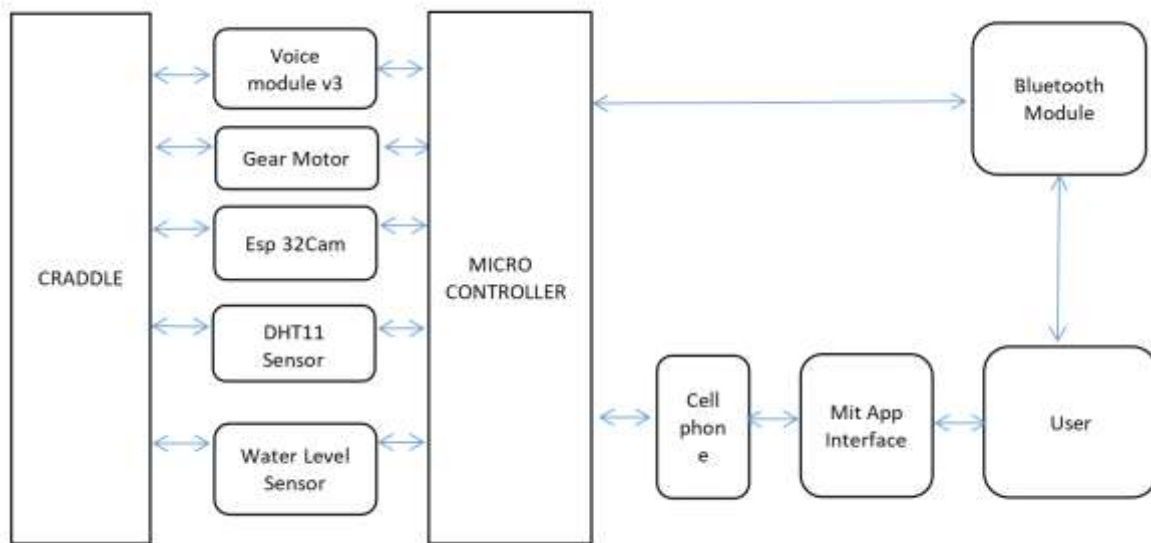
Fig 2: System Architecture
