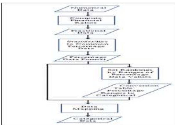
Fig 1:- proposed model
